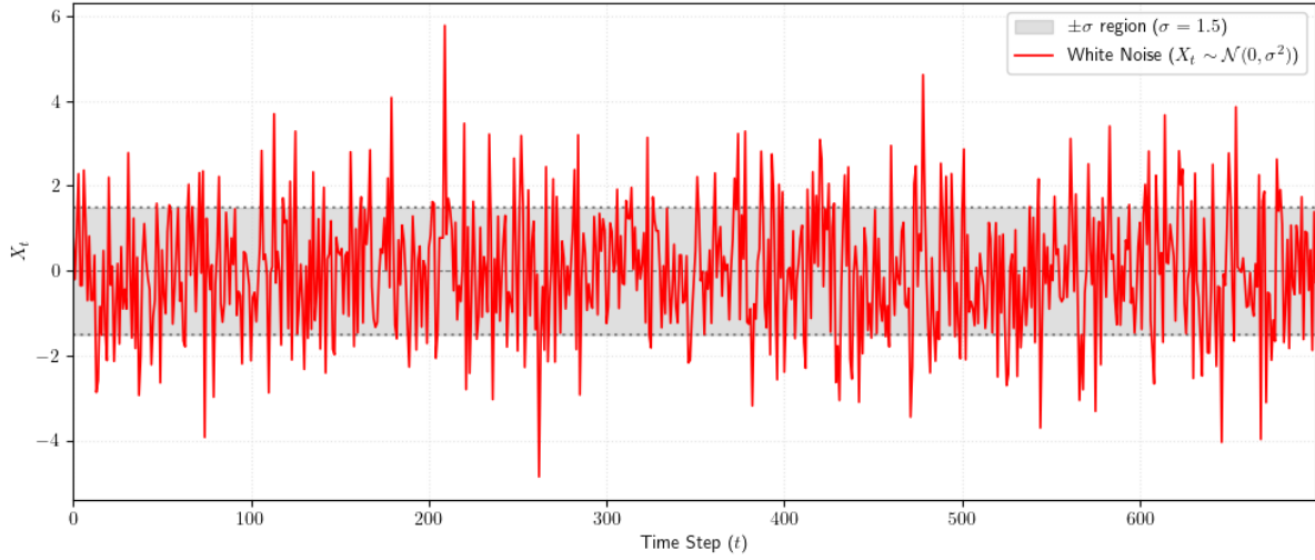
Figure 1.5: A single path of White noise process
