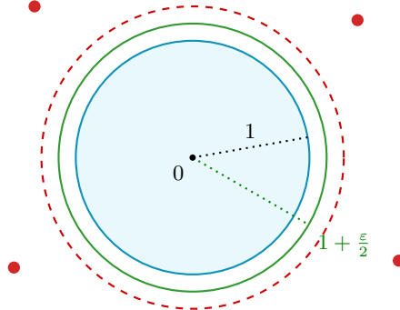
Figure 1.8: The unit circle (solid), the circle of radius 1 + \varepsilon/2 , and the dashed circle of radius 1 + \varepsilon ; the zeros of \phi (red dots) all lie outside the dashed circle.
