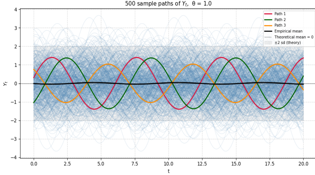
Figure 1.3: Y_t = A \cos(\theta t) + B \sin(\theta t) where A, B \sim \mathcal{N}(0, 1)
