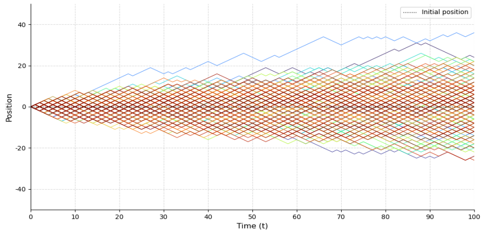
Figure 1.6: Simulation of 250 paths of a Random Walk process
