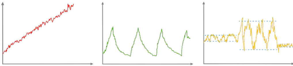
Figure 1.4: Trend , Seasonality , Heteroscedasticity
