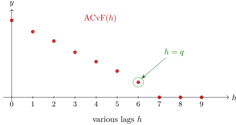
Figure 1.7: Autocovariance function of an MA( q ) process: it vanishes for all lags h > q (here q = 6 ).
